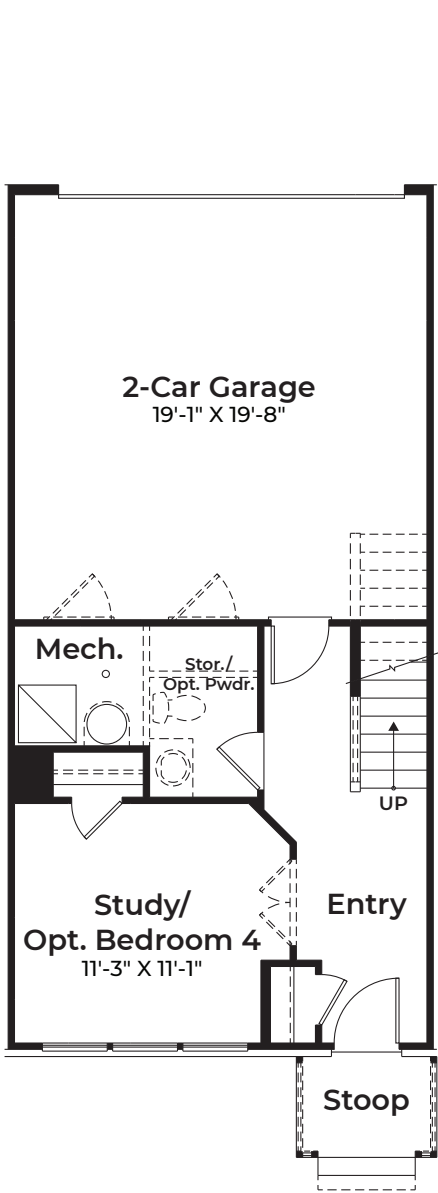
LOWER LEVEL
